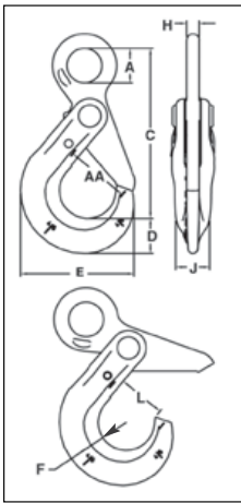
S-1316 EYE HOOK
