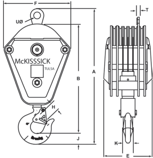
386 – SEXTUPLE
