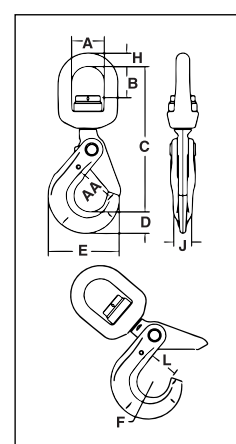
S-13326 SHUR-LOC® Swivel Hook
